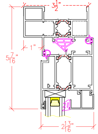
#3 Header Detail
