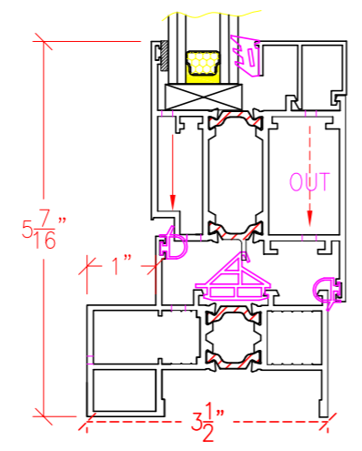
#4 Sill
